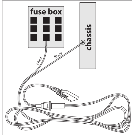
Direct Wiring
